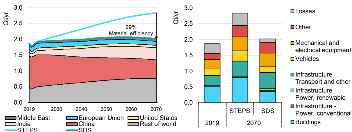
Figure 4.9 Global steel production by region and end use, 2019-70
