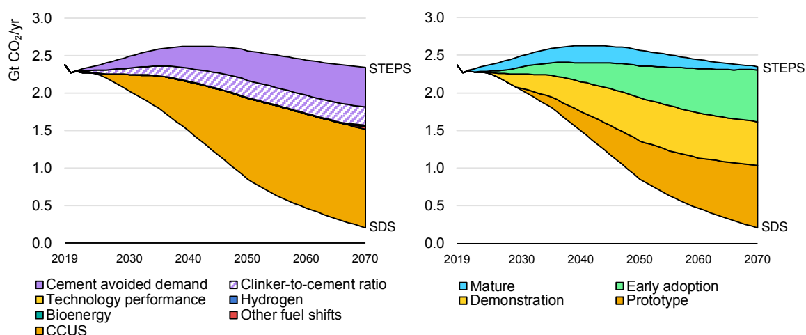
Figure 4.17 Global CO 2 emissions reductions in the cement sector by mitigation strategy and current technology maturity category, 2019-70
