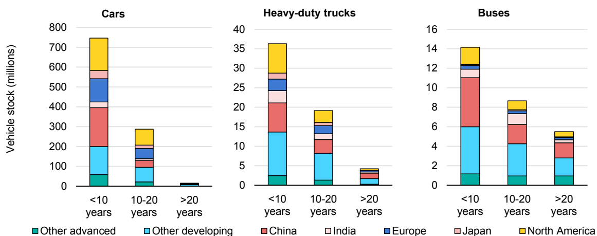
Figure 1.16 Age profile and geographic distribution of road transport vehicles
