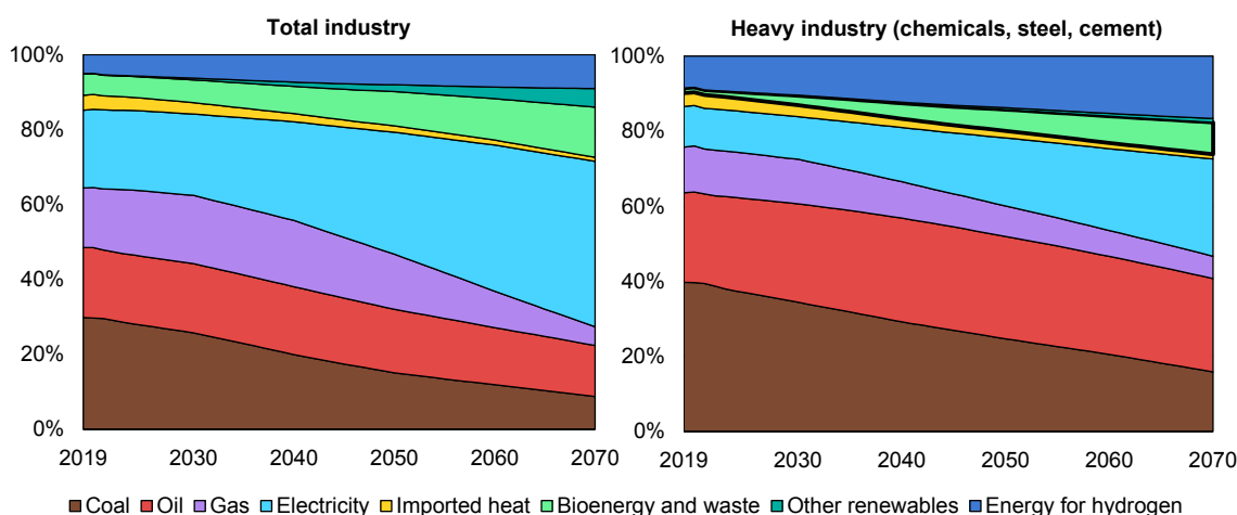
Figure 3.15 Final energy demand by fuel shares for total industry and selected sub-sectors in the Sustainable Development Scenario, 2019-70
