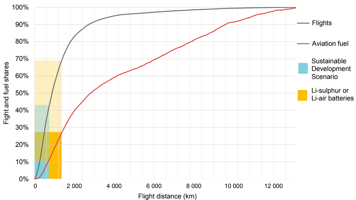
Figure 5.17 Share of flights and fuel use in overall commercial passenger aviation, 2017
