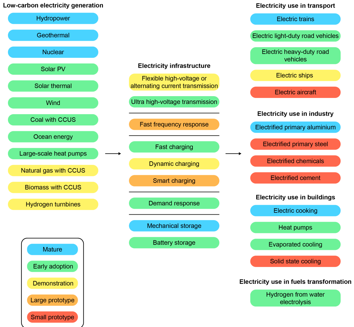
Figure 2.11 Technology readiness level of technologies along the low-carbon electricity value chain
