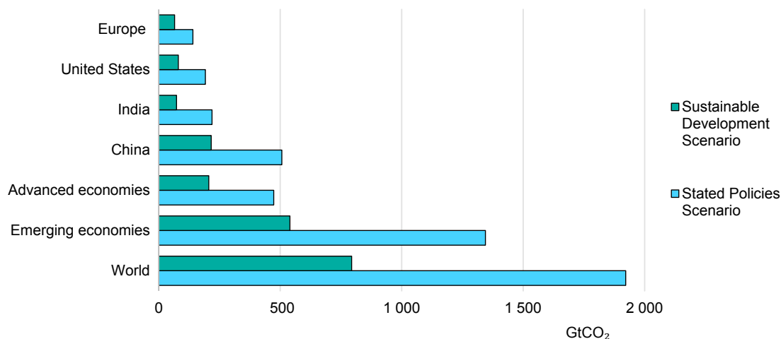
Figure 2.4 Cumulative energy sector CO 2 emissions by region and scenario, 2019-70
